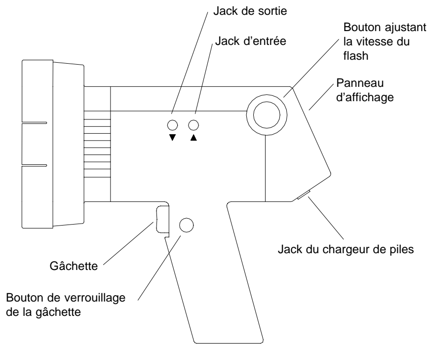
Figure 1 - Stroboscope
