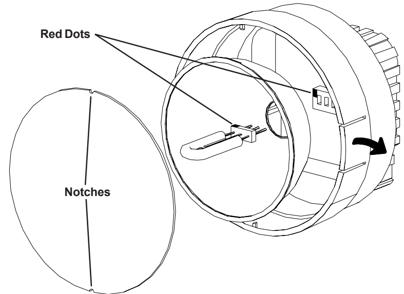
Figure 2 Lamp Replacement
