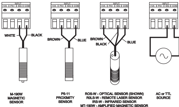
Figure 3 Sensor Connections
