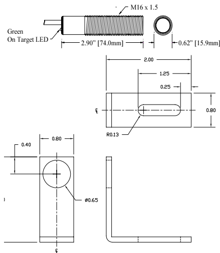
ROS-P and mounting bracket Dimensions
